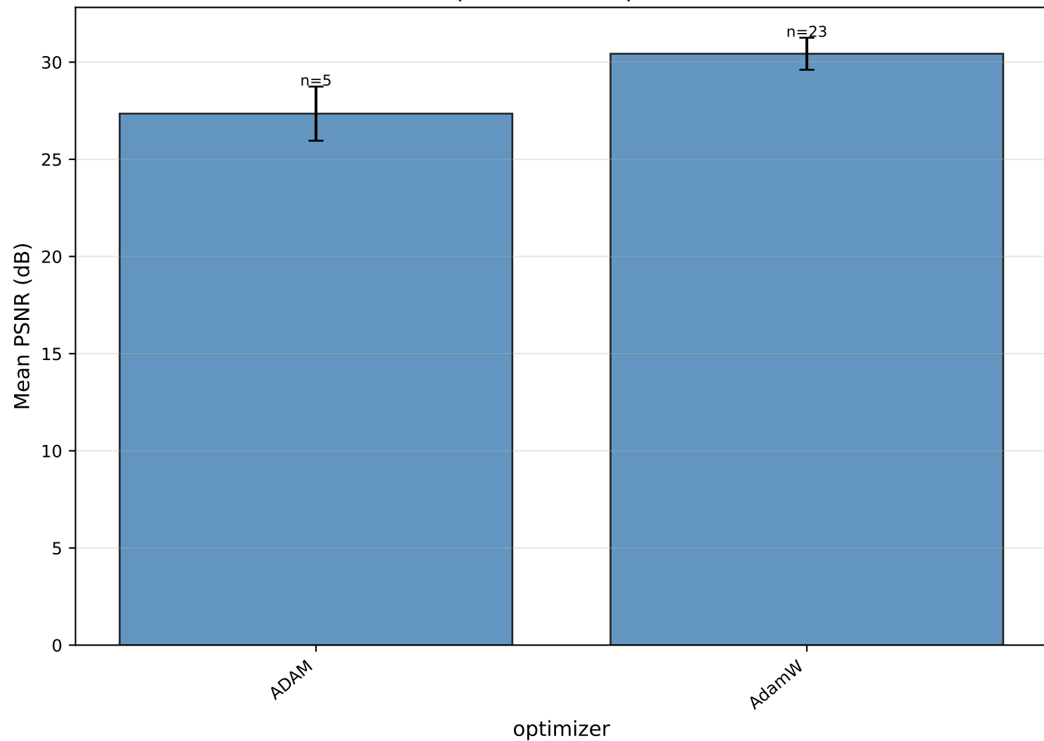
Mean PSNR per value of optimizer — HAT
